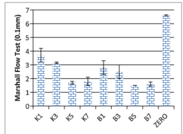
Fig. 9 The results of Marshall test
