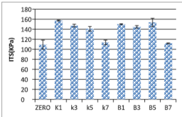
Fig. 8 the results of moisture damage test
