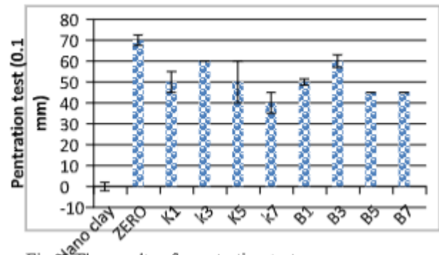
Fig. 5 The results of penetration test .
