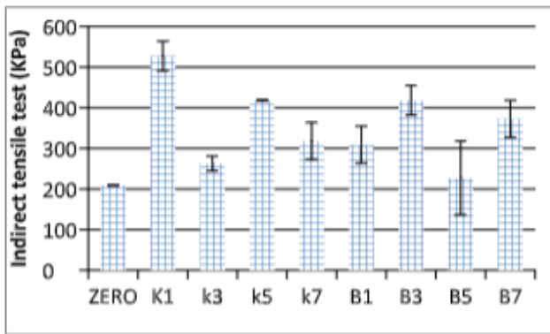
Fig. 7 the results of indirect tensile test
