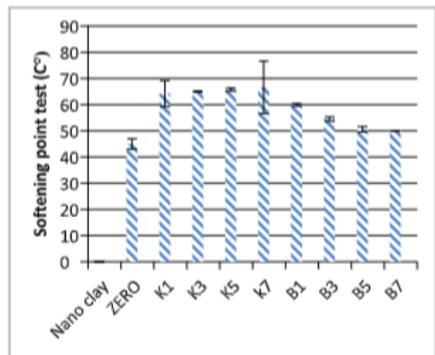
Fig. 6 the results of softening point test
