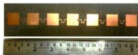
Fig. 3. 7 element Fabricated series antenna array [60]
