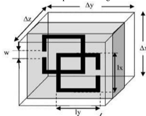
Fig. 2. Geometry of a patch antenna covered by an engineered magnetic superstrate [59]
