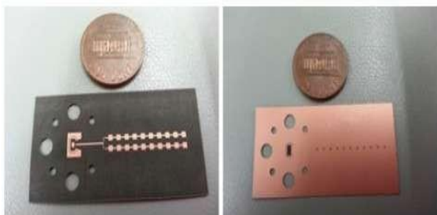
Fig.1. Fabricated antenna with CSRR [50]
