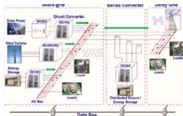
Fig(1):hybrid architecture of a grid connected renewable energy sources
